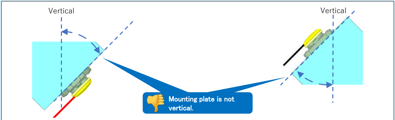
Incorrect Mounting – Mounting bulkhead not vertical
