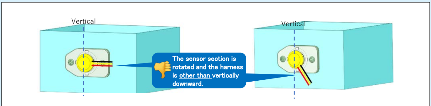
Incorrect Mounting – Sensor assembly twisted – sensor harness and cable should be directed vertically downward
