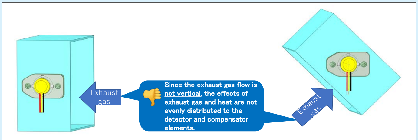
Incorrect Mounting – Sensor Mounted horizontally but direction of gas flow not vertical
