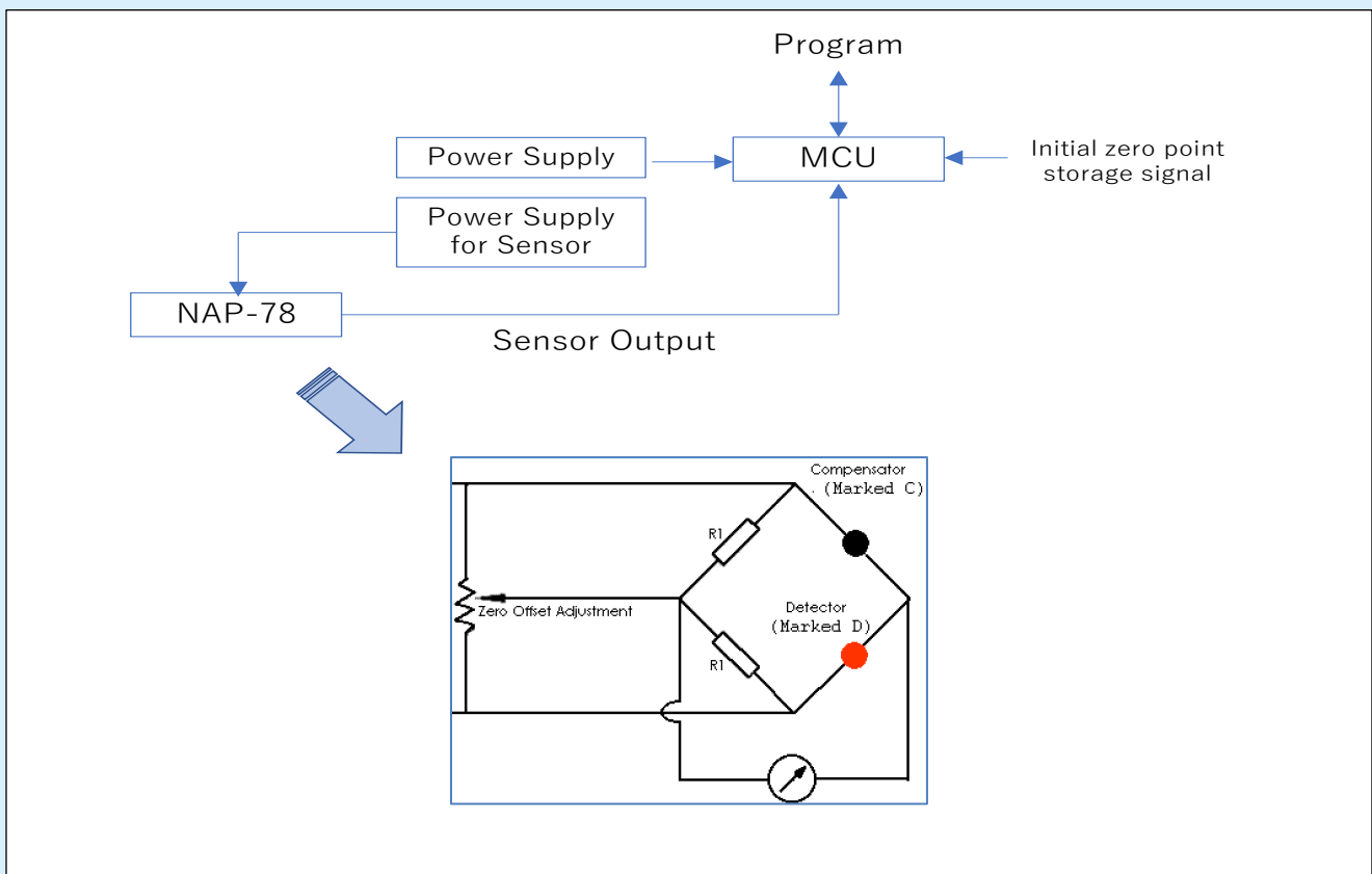
Typical schematic layout within an appliance
