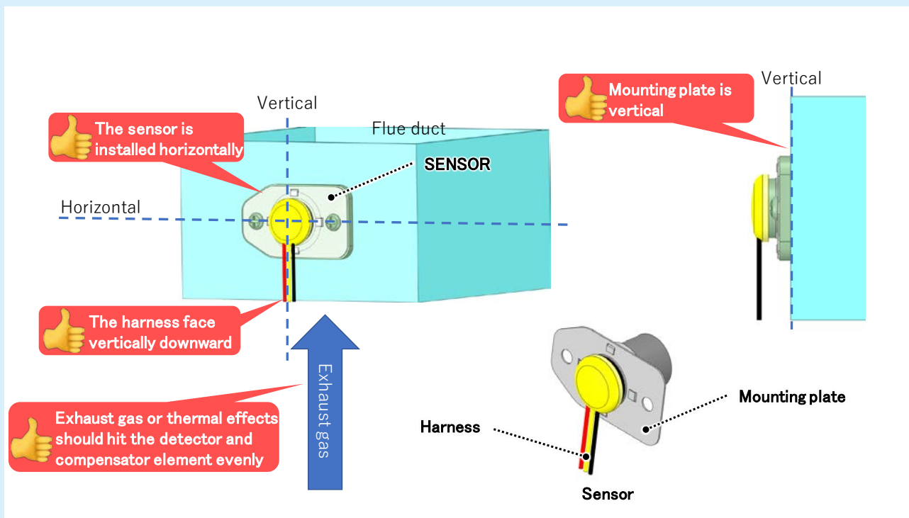
Correct Mounting Of the NAP-78SU
